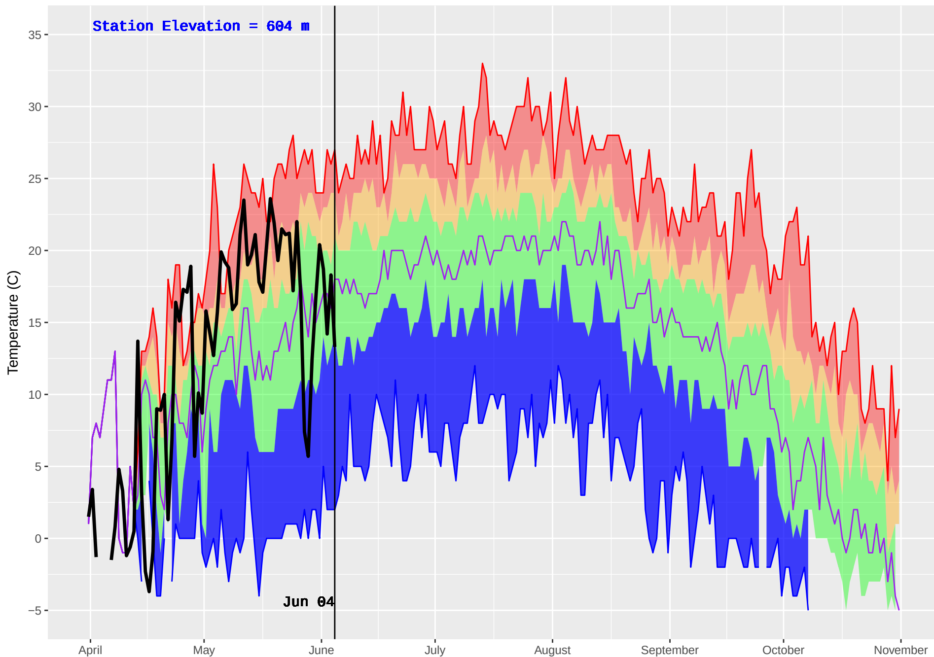
NELSON FORKS (119) : Historical (1986–2016) and Current (2018) Noon Temperature
