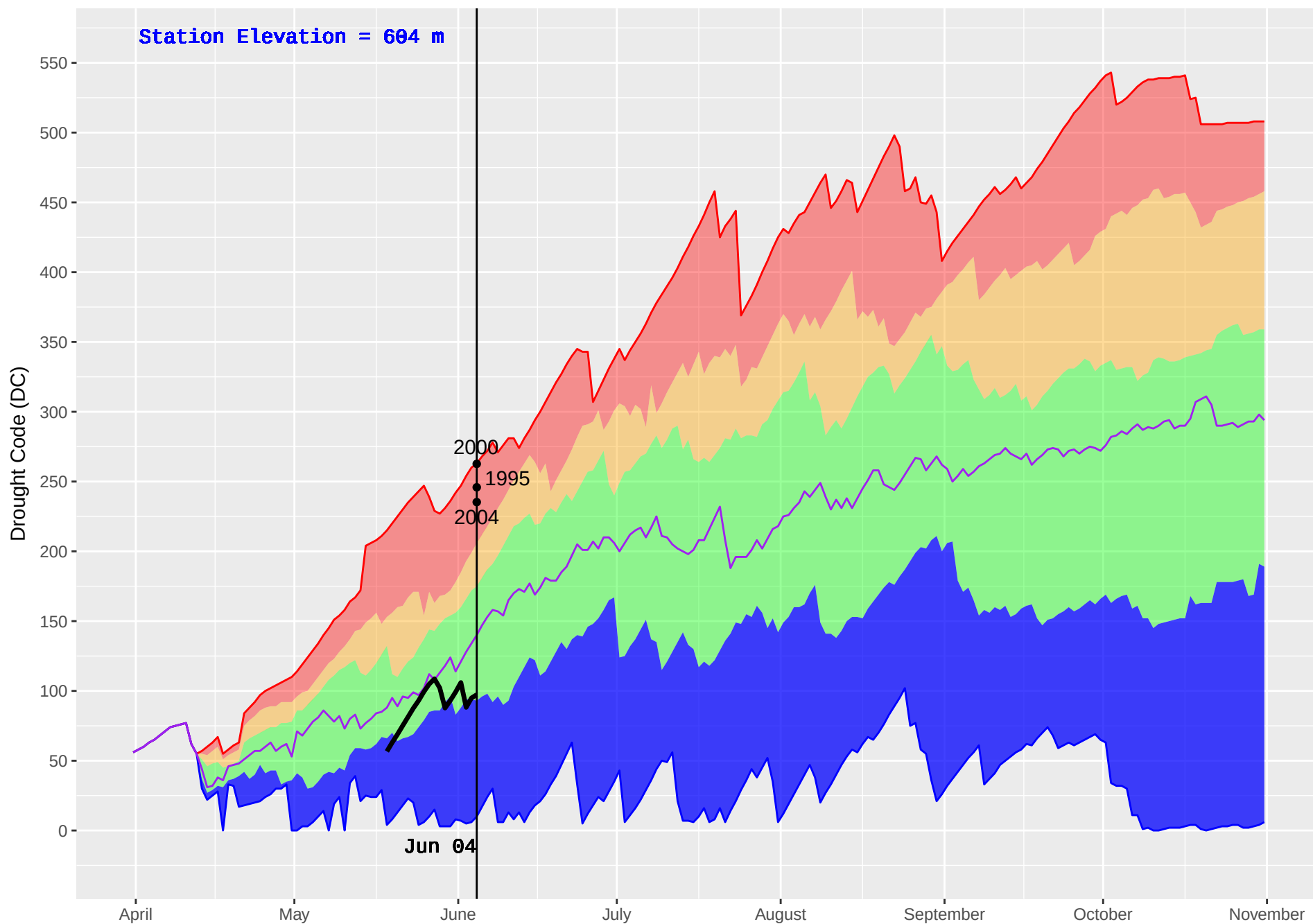
NELSON FORKS (119) : Historical (1986–2016) and Current (2018) Noon Drought Code (DC)
