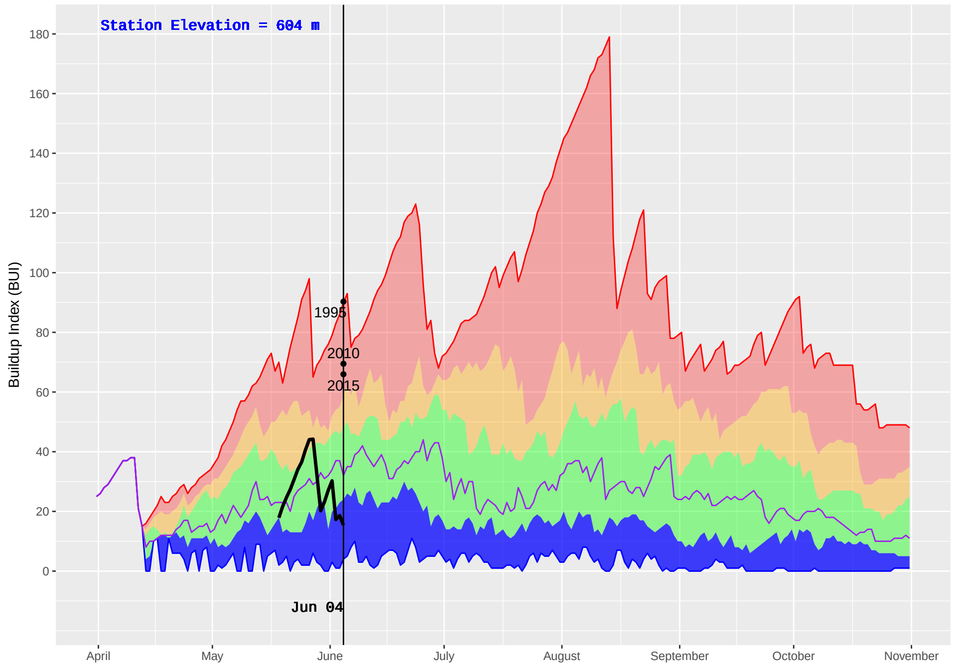
NELSON FORKS (119) : Historical (1986–2016) and Current (2018) Noon Buildup Index (BUI)
