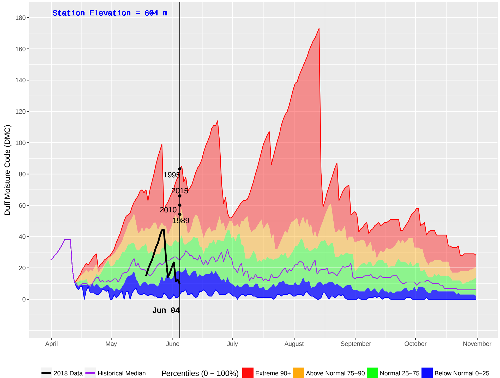
NELSON FORKS (119) : Historical (1986–2016) and Current (2018) Noon Duff Moisture Code (DMC)
