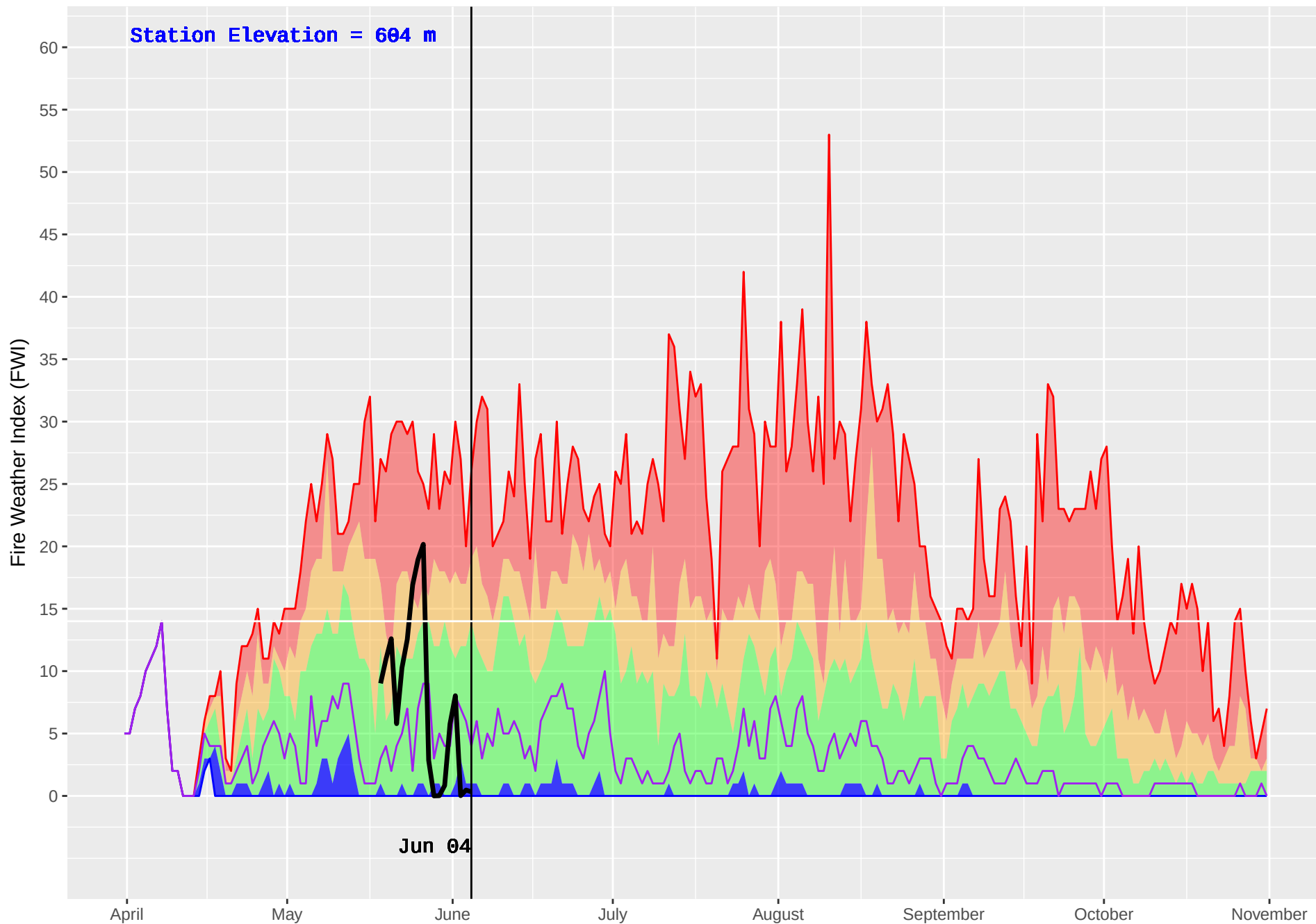
NELSON FORKS (119) : Historical (1986–2016) and Current (2018) Noon Fire Weather Index (FWI)
