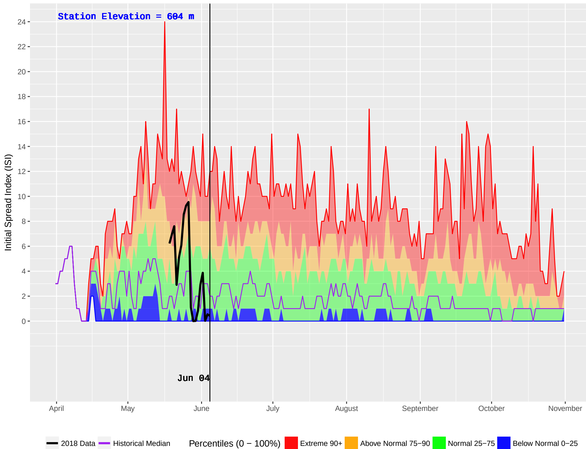
NELSON FORKS (119) : Historical (1986–2016) and Current (2018) Noon Initial Spread Index (ISI)
