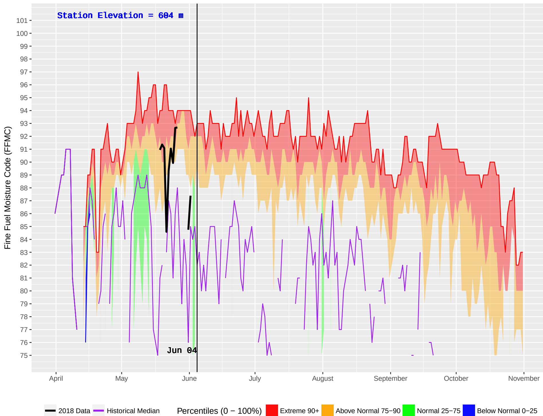
NELSON FORKS (119) : Historical (1986–2016) and Current (2018) Noon Fine Fuel Moisture Code (FFMC)
