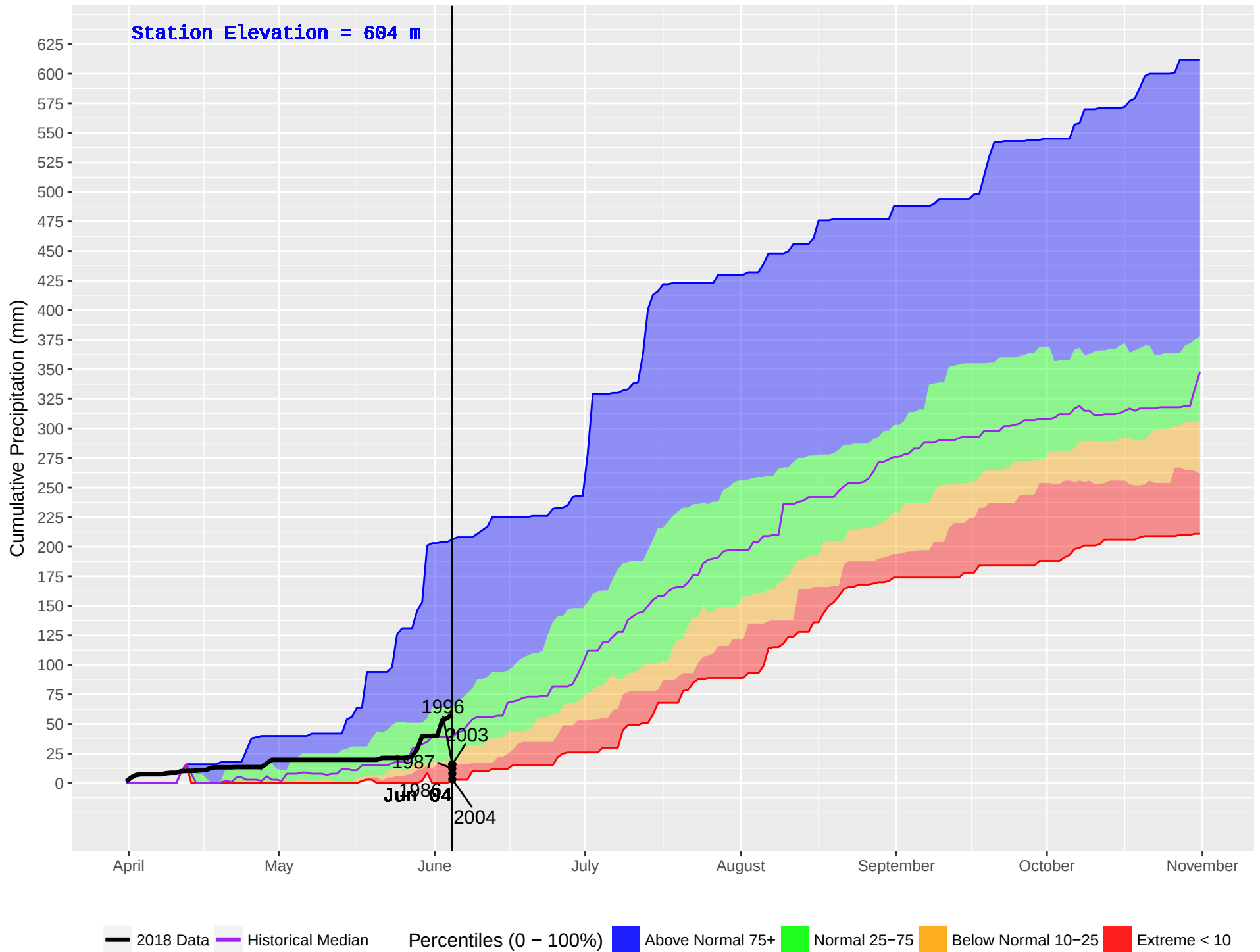
NELSON FORKS (119) : Historical (1986–2016) and Current (2018) Noon Cumulative Precipitation
