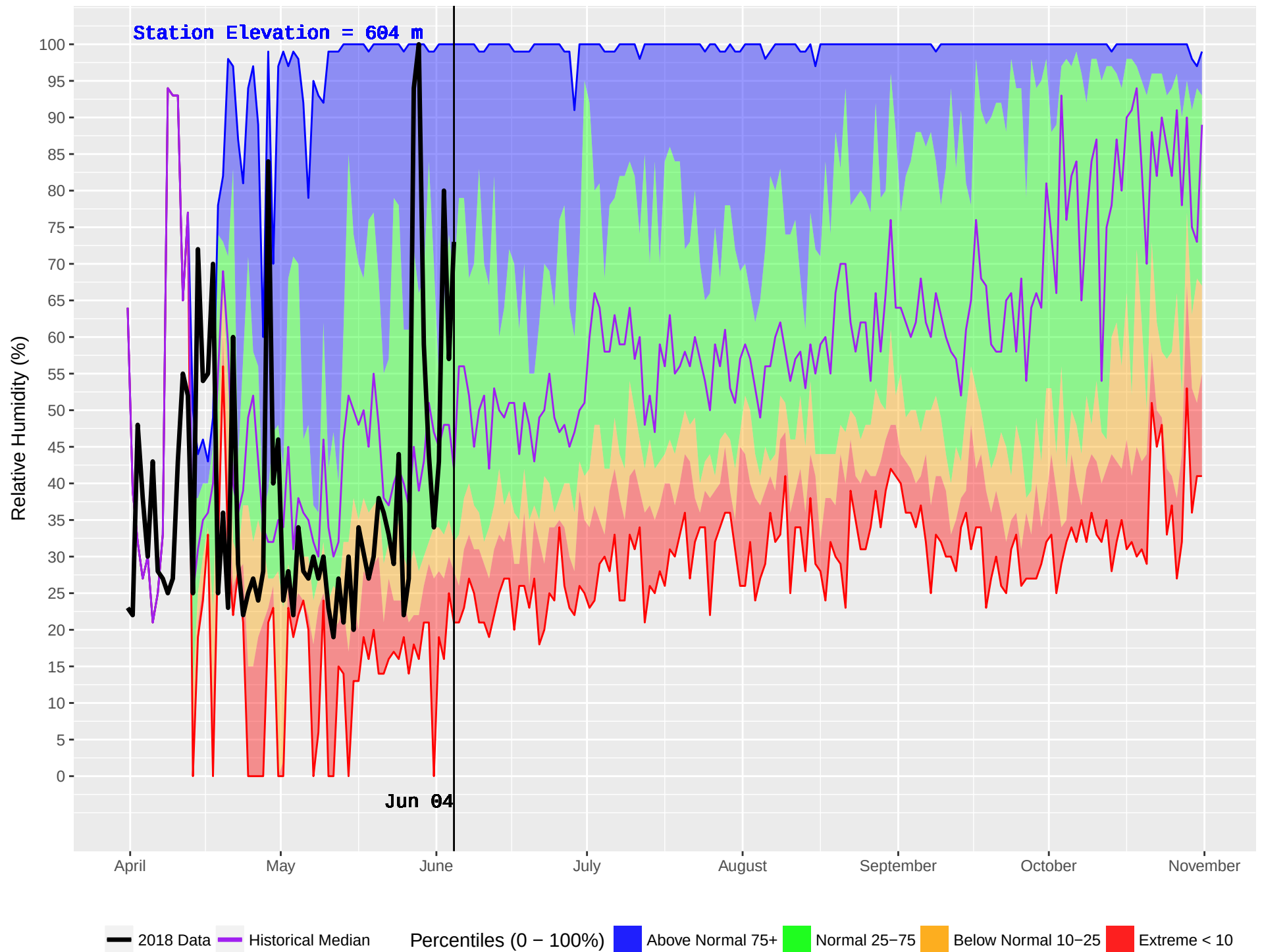
NELSON FORKS (119) : Historical (1986–2016) and Current (2018) Noon Relative Humidity
